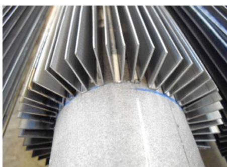
Finned pipe 4" XS A106
